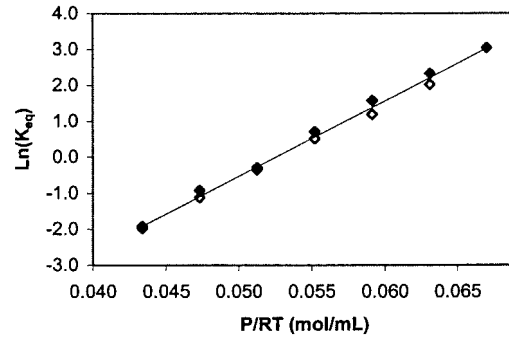
Fig. 3. \ln(K_{eq}) vs. P/RT for the equilibrium transition of rhIFN- \gamma in 0 M sucrose buffer monitored by 2D UV at 32°C. Concentrations of 0.5 mg/ml ( \diamond ) and 1.1 mg/ml ( \blacklozenge ) were run to determine whether the equilibrium process monitored was concentration dependent. Overlap of the data sets indicates the event is consistent with dissociation.
